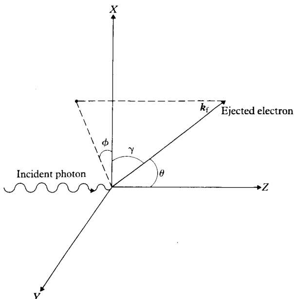
4.7 The angles employed in the discussion of the photoelectric effect. The incident radiation is in the Z direction, with polarisation vector in the X direction. The momentum of the ejected electron is \hbar\mathbf{k}_f .
